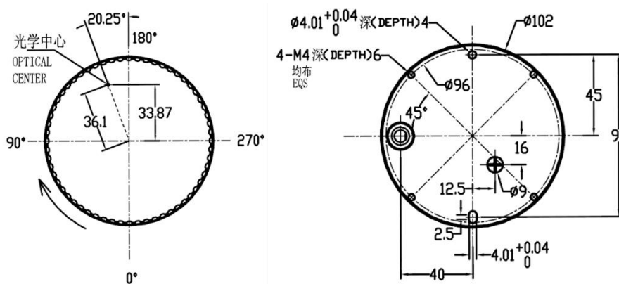
Figure 1.6 C32 Lidar Base (unit: mm) (cable interface at bottom)
