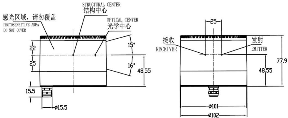
Figure 1.8 C32 Mechanical Drawing (unit: mm) (cable interface at bottom)
