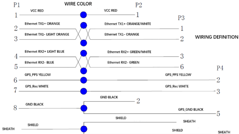
Figure 2.3 Wiring Definition of the Adapter Cable
