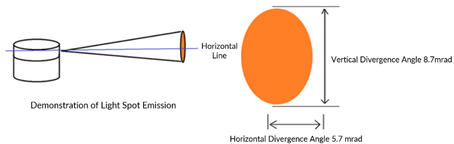
Figure 1.9 Light Spot Demonstration
