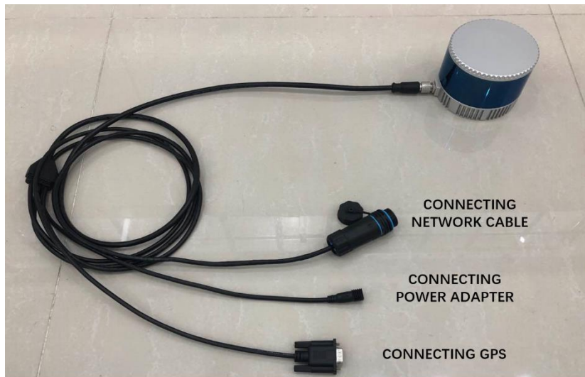
Figure 3.1 Connecting Lidar and Computer
