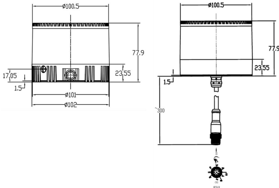
Figure 1.4 C32 Dimensions (unit: mm) (left: side; right: bottom)
