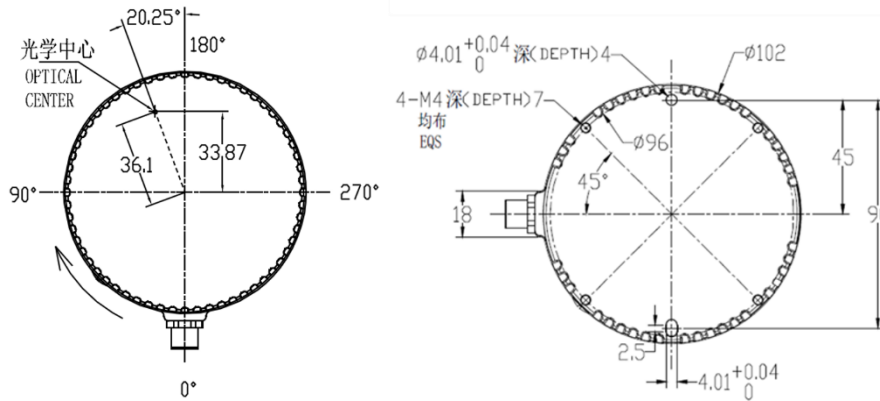
Figure 1.5 C32 Lidar Base (unit: mm) (cable interface at side)
