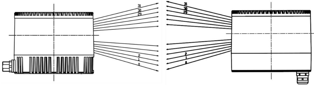
Figure 1.2 Laser Beam Distribution (left: side; right: bottom)
