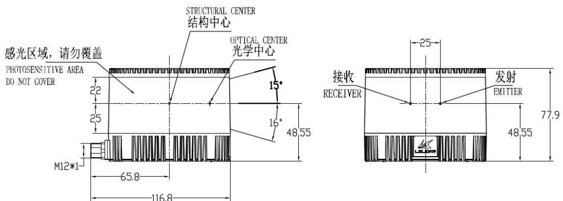
Figure 1.7 C32 Mechanical Drawing (unit: mm) (cable interface at side)
